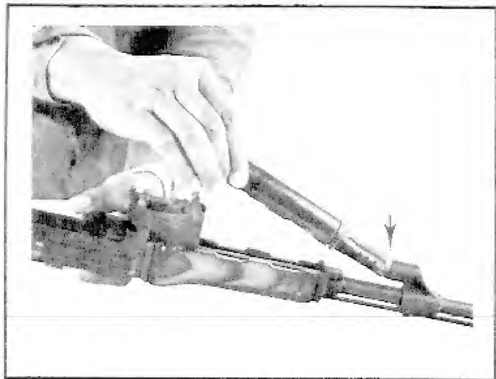
FIGURE 35. ENGAGING TUBE
